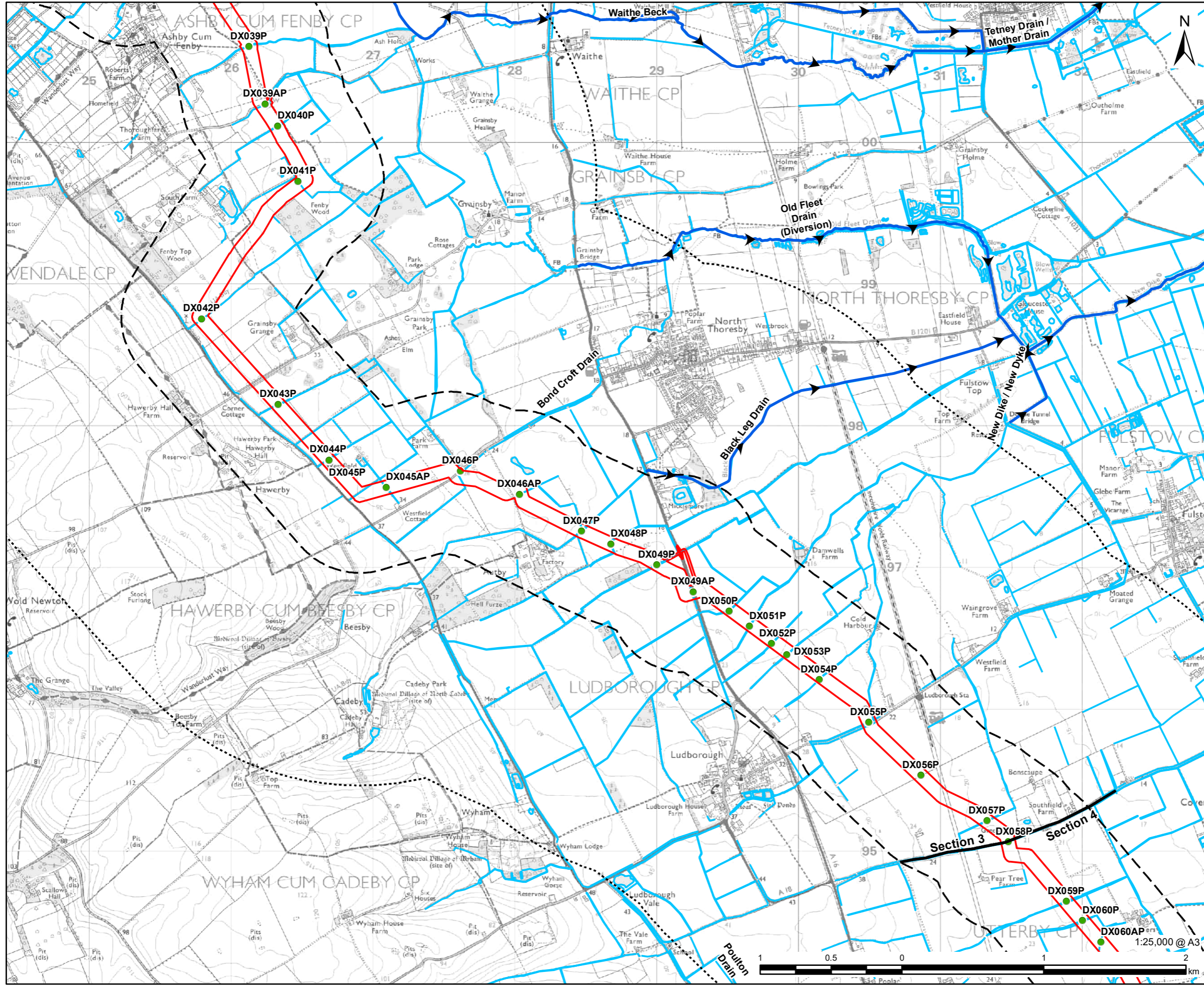
FIGURE TITLE Figure 11-2 (4 of 7) Watercourse Details showing Crossing Reference and Flow Direction
